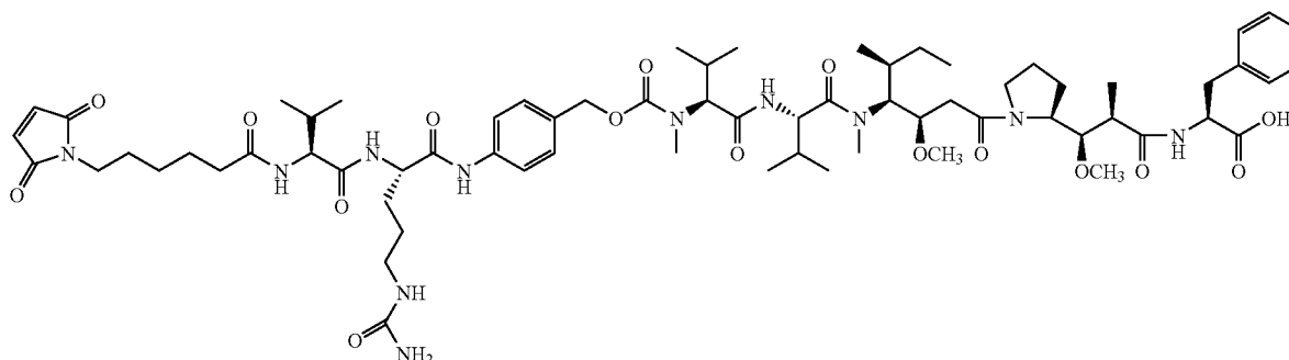
MC-val-cit-PAB-MMAF
